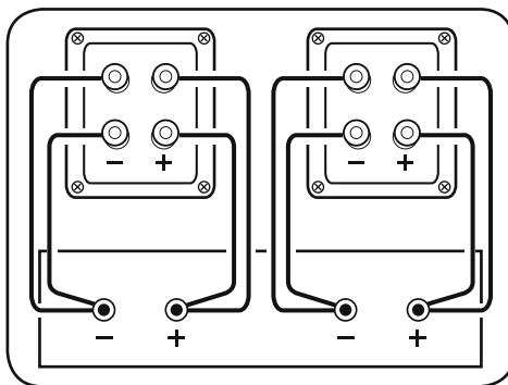
Bi-Wiring
